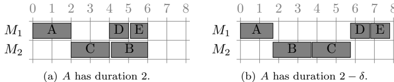
Figure 1: Consider tasks A , B , C of duration 2 and D , E of duration 1, to be scheduled on two machines. As usual, we assume that a machine can execute a single task at a time. Dependences between tasks are as follows: A \rightarrow B and C \rightarrow D, E , meaning e.g. that A must be completed before B can start. Task A must be executed on machine M_1 and tasks B , C on machine M_2 . Moreover, the release time of task C means that it cannot be scheduled before 2 time units. Fig. 1(a) shows the optimal greedy schedule for these tasks under these constraints, while Fig. 1(b) shows the outcome of any greedy scheduler when the duration of task A is less than 2.
