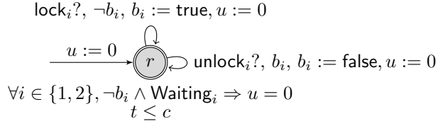
Figure A.19: Timed automaton \mathcal{M} ensuring mutual exclusion and greedy scheduling.
