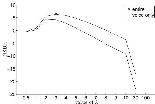
Figure 1: Variation of the estimated singing voice NSDR (see definition in Section 4) according to the value of \lambda under two situations. •: NSDR when only the singing voice-active parts of the separated signal are processed. *: NSDR when the entire signal is processed.
