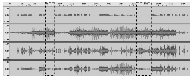
Figure 3: Separated voice for various values of \lambda for the Pink Noise Party song Their Shallow Singularity . From top to bottom: clean voice, constant \lambda_1 = 1/\sqrt{\max(m, n)} , constant \lambda = 5 * \lambda_1 , adaptive \lambda = (\lambda_1, 5 * \lambda_1) .
