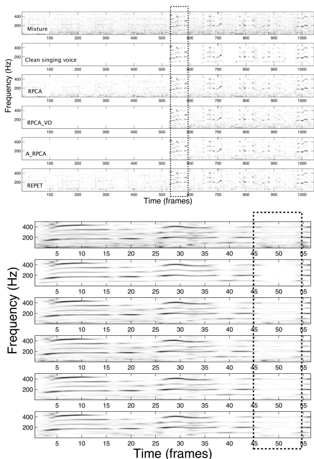
Figure 4: [Top Figure] Example decomposition on an excerpt of the Doobie Brothers song Long Train Running and [Bottom Figure] zoom between frames [525-580] (dashed rectangle in the Top Figure). For each figure, the top pane shows the part between 0 and 500Hz of the spectrogram of the original signal. The clean singing voice appears in the second pane. The separated singing voice obtained with baseline model (RPCA), with the baseline model when restricting the analysis to singing voice-active segments only (RPCA_VO), and with the proposed A-RPCA model are represented in panes 3 to 5. For comparison, the sixth pane shows the results obtained with REPET [16].
