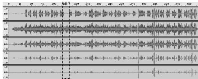
Figure 2: Waveform of the separated voice for various values of \lambda for the song Is This Love by Bob Marley. From top to bottom: clean voice, \lambda = \lambda_1, 2 * \lambda_1, 5 * \lambda_1, 10 * \lambda_1 .
