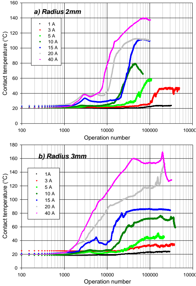
Fig.5. Contact temperature versus cycle number for three currents: a) Radius 2mm; b) Radius 3mm
