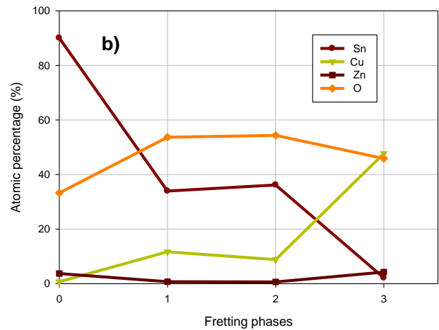
Fig.8. Fretting zone and microscopic analysis of elements Sn, Cu, Zn, O. a) Fretting zone photography showing debris b) Atomic percentage of elements at Phase 1, 2 and 3 (0 is no fretted zone)
