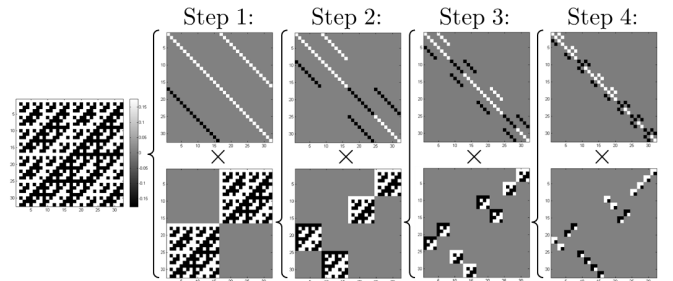
Fig. 2. Hierarchical factorization of the Hadamard matrix of size 32 \times 32 . The matrix is iteratively factorized in 2 factors, until we have Q = 5 factors, each having p = 64 non-zero entries.
