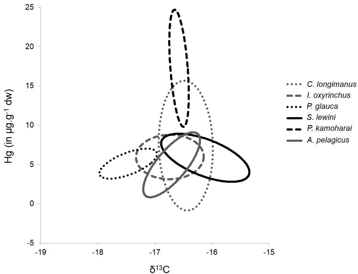
Fig. 5. Standard ellipses for corrected sample sizes (SEAc, in ‰, \delta^{13}\text{C} ) and Hg concentrations (in \mu\text{g}\cdot\text{g}^{-1} dw) of A. pelagicus , C. longimanus , P. glauca , S. lewini , I. oxyrinchus and P. kamoharai .
