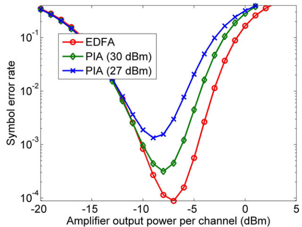
Figure 15 Symbol error probability versus the amplifier output power per channel for EDFA and PIA with different pump powers (100 × 28 GBd 16-QAM WDM Chs, 10 × 75 km fiber spans, 50-GHz grid).
