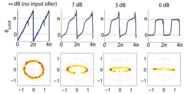
Figure 20 Signal phase (top) at PSA output versus input phase for different idler powers and corresponding complex plane constellation diagrams (bottom), in which the x- and y-scale represent normalized real and imaginary parts of the electric field.
