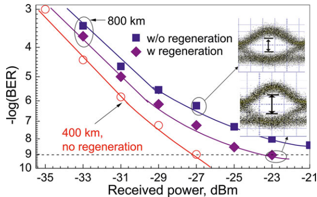
Figure 9 BER curves (and eye diagrams) of a DPSK signal after transmission over 400 km and 800 km of fiber, with and without PSA-based regeneration.
