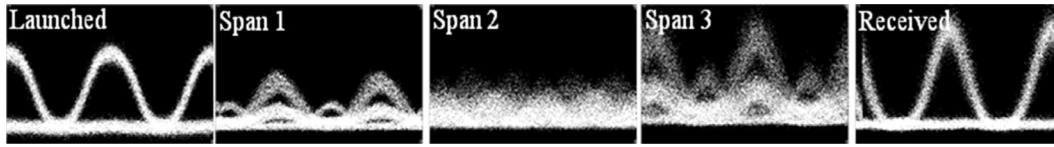
Figure 24 WDM transmission compensated by polarization-invariant mid-link compensator: typical channel waveform (10Gb/s) at launch, and interim spans of the link [81].
