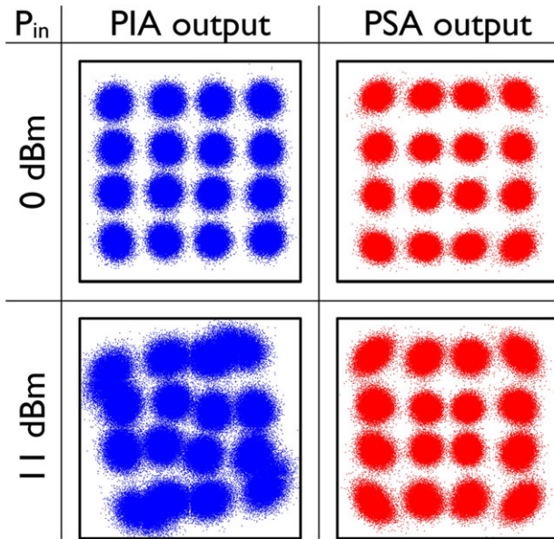
Figure 22 Constellation diagrams of 40Gbit/s 16-QAM signal after 105 km transmission at low power (0 dBm – top row) and high power (11 dBm – bottom row) for phase-insensitive (left) and phase-sensitive (right) amplification.
