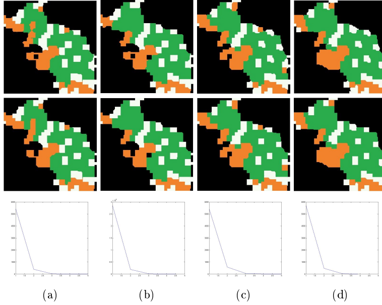
Fig. 7. n -ary processing of Fig. 6 (a). first row: composed n -ary filter \psi(I; B) , second row: iterated composed n -ary filter \psi^k(I; B) until convergence, third row: convergence speed w.r.t. to k . Column (a) \psi(I; B) = \gamma_1 \circ \gamma_2 \circ \gamma_3 \circ \gamma_4 , (b) \psi(I; B) = \gamma_2 \circ \gamma_1 \circ \gamma_3 \circ \gamma_4 , (c) \psi(I; B) = \gamma_3 \circ \gamma_4 \circ \gamma_1 \circ \gamma_2 , (d) \psi(I; B) = \gamma_4 \circ \gamma_3 \circ \gamma_2 \circ \gamma_1 .
