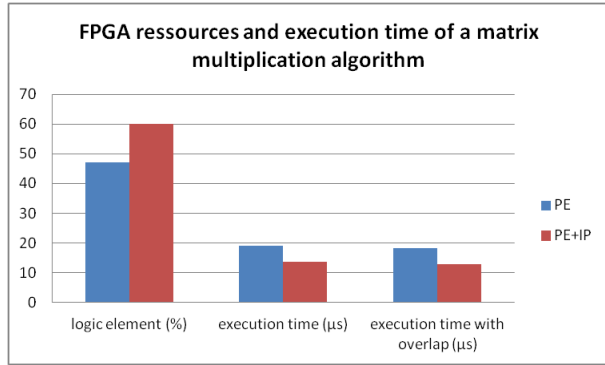
Fig. 4. Experimental results of running a MM algorithm
