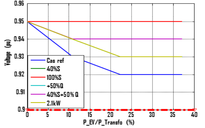
Fig. 16: Minimal voltage for 6 cases
