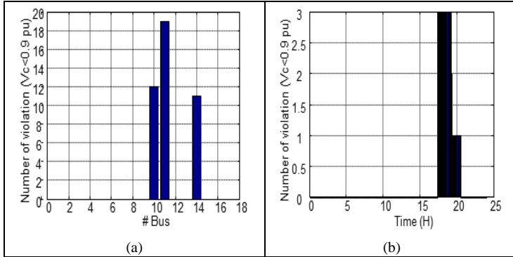
Fig. 10. Distribution of violation in voltage (<0.9 pu)
