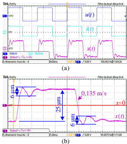
FIG. 15. Transient plot of the voltage v(t) , the current i(t) and the membrane displacement x(t) .
