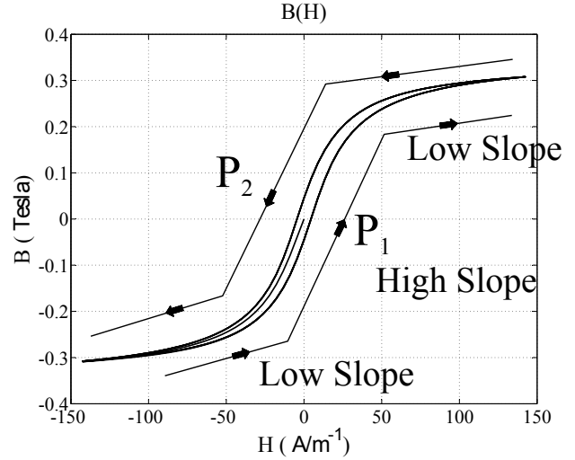
Fig. 7. Magnetic hysteresis loop.
