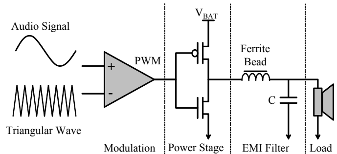
Fig. 1. Basic architecture of Class-D audio amplifier.
