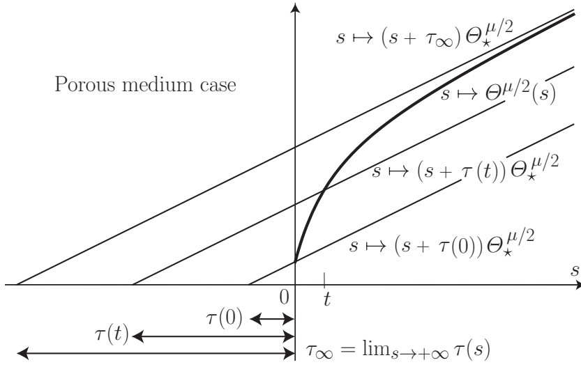
Fig. 2 In the porous medium case, the curve s \mapsto \Theta^{\mu/2}(s) is still increasing but concave, so that t \mapsto \tau(t) is monotone increasing, unless the solution is itself a Barenblatt solution up to a time shift.
