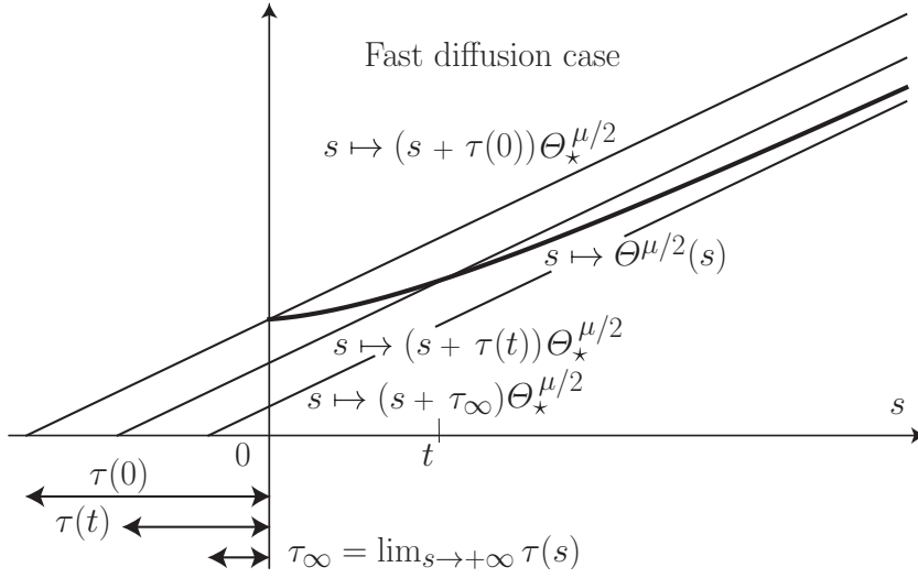
Fig. 1 In the fast diffusion case, the (bold) curve s \mapsto G(s) = \Theta^{\mu/2}(s) is convex, increasing, and its asymptote is s \mapsto (s + \tau_\infty) \Theta_\star^{\mu/2} . At any time t \geq 0 , we observe that it crosses the line s \mapsto (s + \tau(t)) \Theta_\star^{\mu/2} = (s - t + 1) \Theta^{\mu/2}(t) transversally, so that t \mapsto \tau(t) is monotone decreasing, unless the solution is itself a Barenblatt solution up to a time shift.
