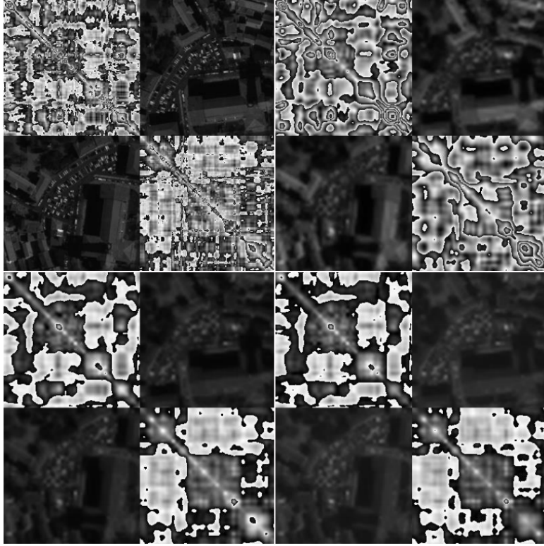
FIGURE 2. Color-coded (white=0, black=max) images of the special form of covariance matrix (10) computed from the high resolution B&W image (top-left), the red component of the low resolution color image (top-right), the green component of the low resolution color image (bottom-left) and the blue component of the low resolution color image (bottom-right).
