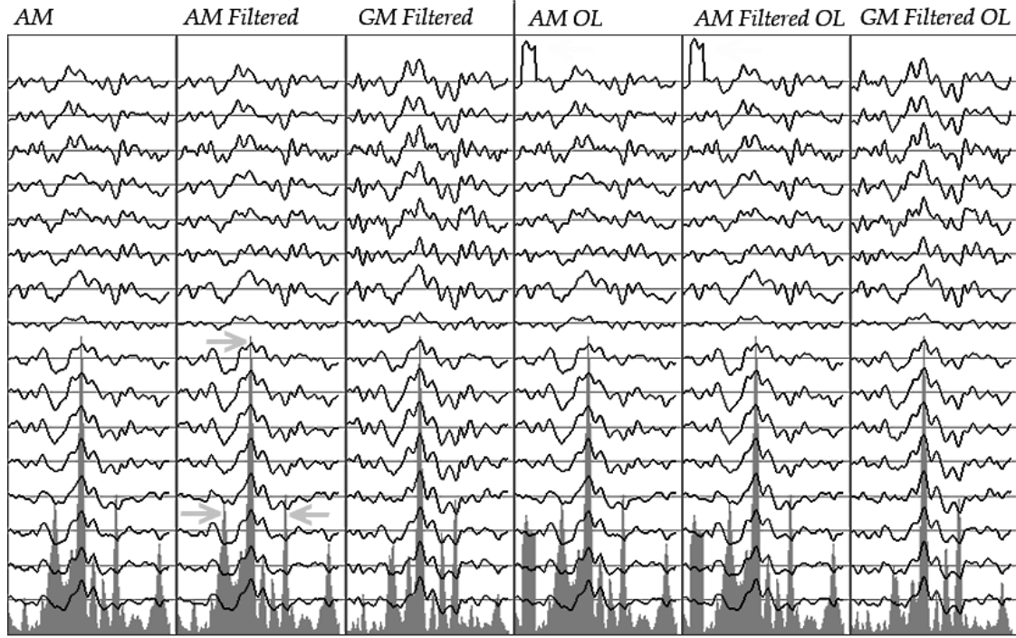
FIGURE 3. 1-sec average ERP estimations for one subject recorded at 16 electrodes. For consistency with neurological convention, a positive voltage deflection is plotted downward. The voltage scale of each plot is arbitrary but consistent within each plot. The shaded grey area is the global field power (GFP), that is, the total energy (sum of the squared potential across electrodes) at each sample. The GFP is scaled arbitrarily in each plot. The first three plots are, from left to right, the arithmetic mean of the raw ERPs \mathbf{X}_i , the arithmetic mean of the ERPs after filtering of the trials as per (12) (given by \mathbf{X}_i \leftarrow \mathbf{U}^T \mathbf{X}_i \mathbf{V} ) and the geometric mean of the trials obtained as the top-right off-diagonal block of the geometric mean of trials represented by (10), ri-expanded in the original dimension by \mathbf{X}_i \leftarrow \mathbf{U} \mathbf{X}_i \mathbf{V}^T . The next three plots are the same three mean estimations obtained with the outlier, which is well visible at the beginning of the trace of the first electrode only in the arithmetic means.
