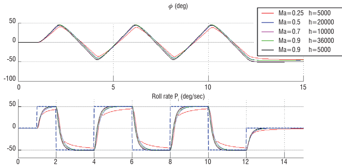
Figure 4 - Nonlinear simulations for various flight conditions: lateral axis
