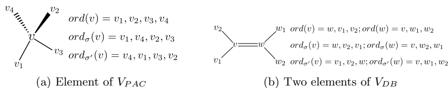
Fig. 2: Example of elements of V_{PAC} and of V_{DB} with their ordered list (top) and the ordered lists obtained using two permutations \sigma and \sigma'
