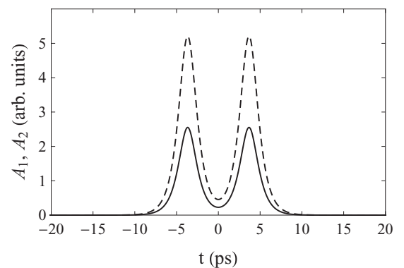
FIG. 12. Double-humped pulse pair as a solution of Eq. (70), A_1(t) (lower curve) and A_2(t) (upper curve): \theta_1 = 2\pi , \theta_2 = 4\pi , \delta = 3.82 , v = 1.04 , \kappa = 0.36 .
