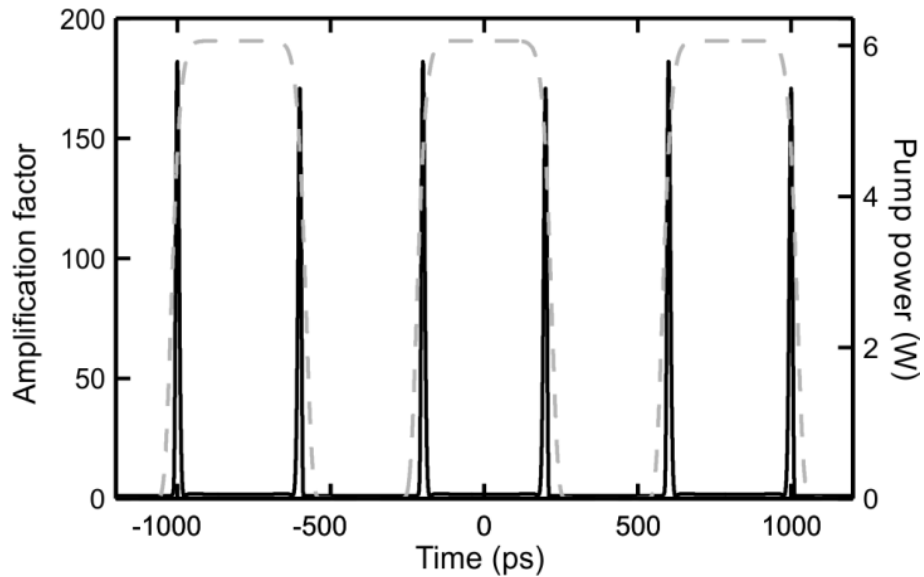
Figure 9 : Amplification factor experienced by the CW seed (solid black curves) compared against the temporal pump power profile (dashed grey curves) for a super-Gaussian pump pulse train similar to Fig. 7(a) at the repetition rate of 1.25 GHz.
