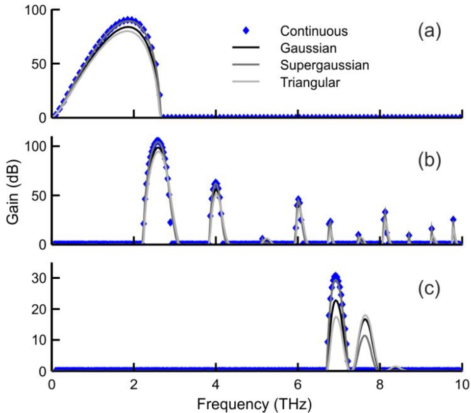
Figure 4 : Details of the output spectra obtained for pulsed pumps having a common peak power of 5.6 W. Results obtained with a Gaussian, super-Gaussian and triangular shapes (black, dark grey and light grey solid lines respectively) are compared with results predicted by the LSA for the CW case (blue diamonds). MI spectra obtained in fibers A, B and C are plotted in panels (a), (b) and (c), respectively.
