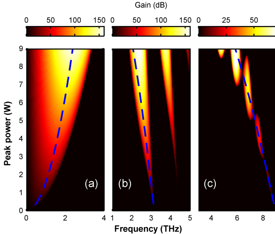
Figure 2 : Evolution of the MI gain profile g(P, \omega) according to pump power P for a CW (a) Analytical results from Eq. 2 in the case of fiber A. Blue line denotes the maximum MI frequency as predicted by Eq. 4. (b-c) Results obtained from the LSA using the Floquet approach for fibers B and C respectively. The resonant frequency predicted by Eq. 6 is denoted by a blue dashed line.
