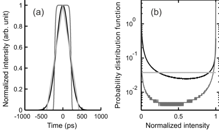
Figure 3 : (a) Comparison of the three temporal intensity profiles of the pulses under investigation : (b) Probability distribution function associated with these profiles (the temporal span of the simulations is 2 ns). Gaussian, super-Gaussian and triangular shapes are plotted using black solid, grey solid and light grey solid lines, respectively.
