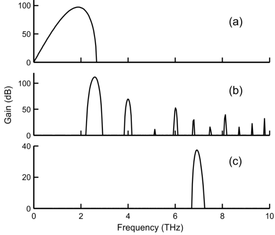
Figure 1 : Evolution of the MI gain profile at the fiber output for a CW pump power P=5.6 W in fibers A, B and C (subplots a, b and c respectively).
