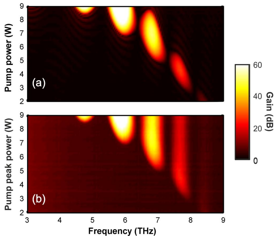
Figure 6 : Evolution of the first QPM band according to pump power according for (a) a continuous pump and (b) a Gaussian pump. Results are obtained from the numerical integration of the NLSE.
