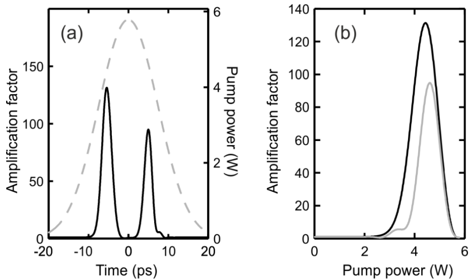
Figure 10 : (a) Amplification factor experienced by the CW seed pulse (solid black curves) compared against the temporal pump power profile (dashed grey curves) for 17.5 ps FWHM duration Gaussian pump pulses. (b) Amplification factor versus instantaneous pump power for signal pulses generated at the leading edge (solid black curve) or the trailing edge (grey curve) of the pump pulse.
