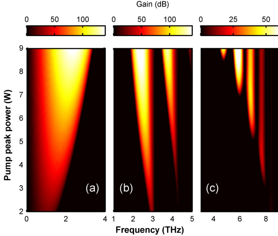
Figure 5 : Evolution of the MI gain profile g(P, \omega) according to the peak power P for a Gaussian pulse in fiber A, B and C (panels a, b and c).
