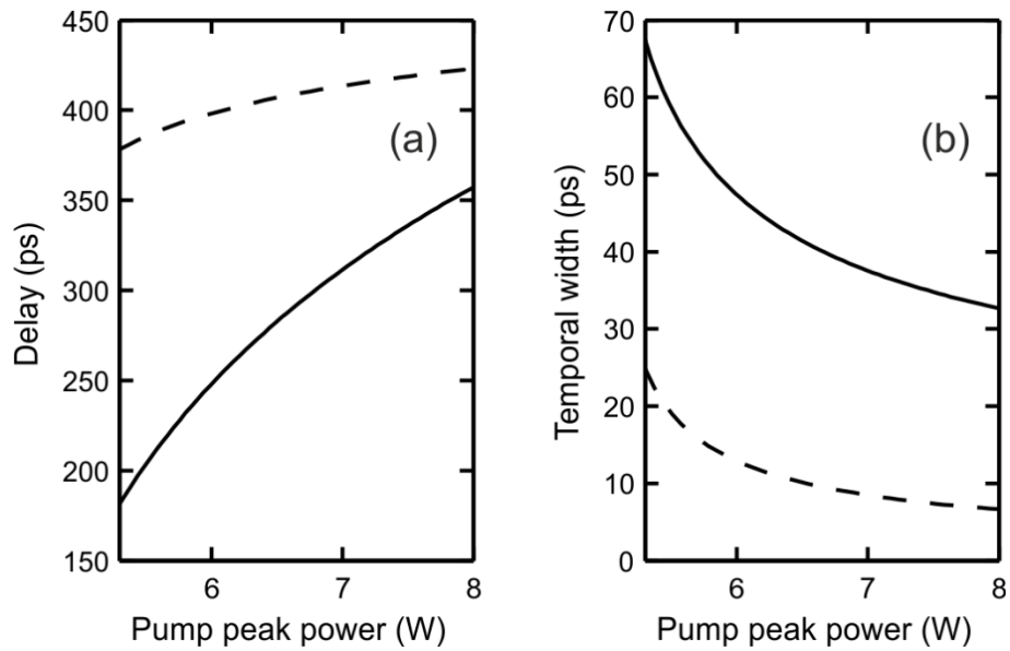
Figure 12 : Evolution of the time delay among the two pulses obtained from the seed (a) and of the FWHM temporal width of the individual pulses (b) vs. the pump peak power for either a Gaussian (black curves) or a super-Gaussian (dashed curves) pump pulse shape.
