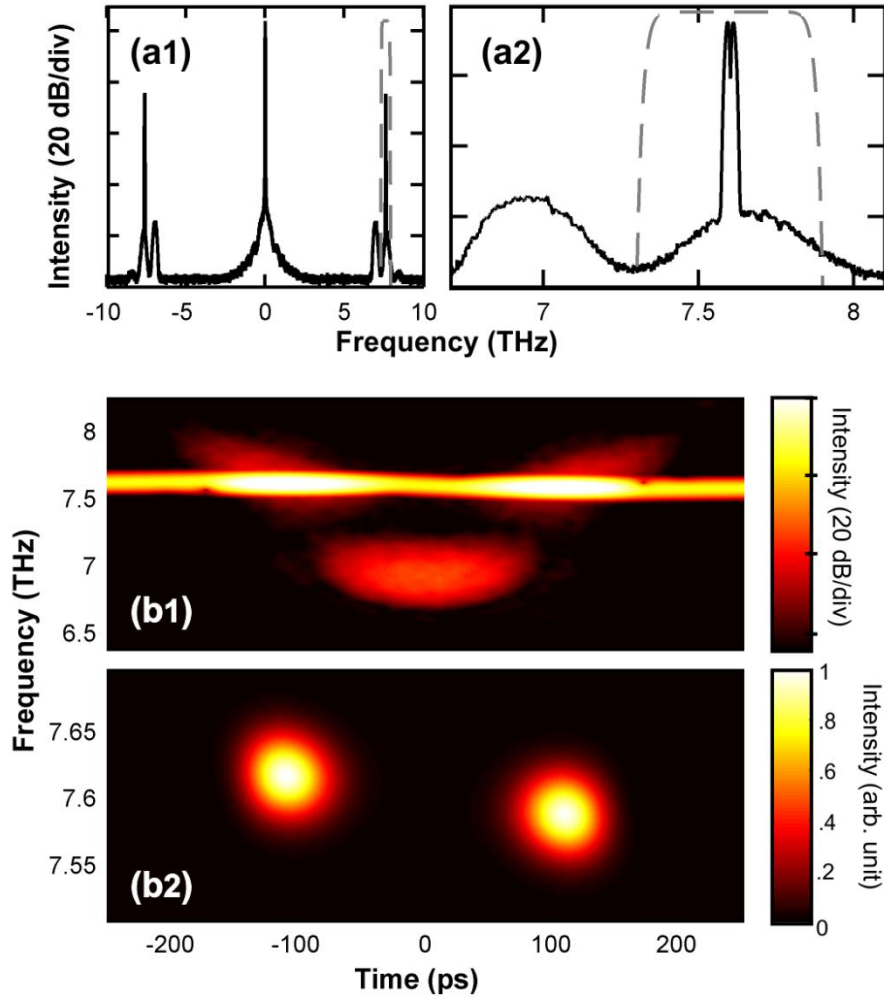
Figure 8 : (a) Optical spectrum of the amplified seed when pumped by a 400-ps Gaussian pulse (black curve) and optical band pass filter used to isolate the amplified seed (grey line). Plot (a2) is a magnification of plot (a1). (b) Spectrogram of the amplified seed on a logarithmic scale (b1) and its magnification with results on a linear scale (b2).
