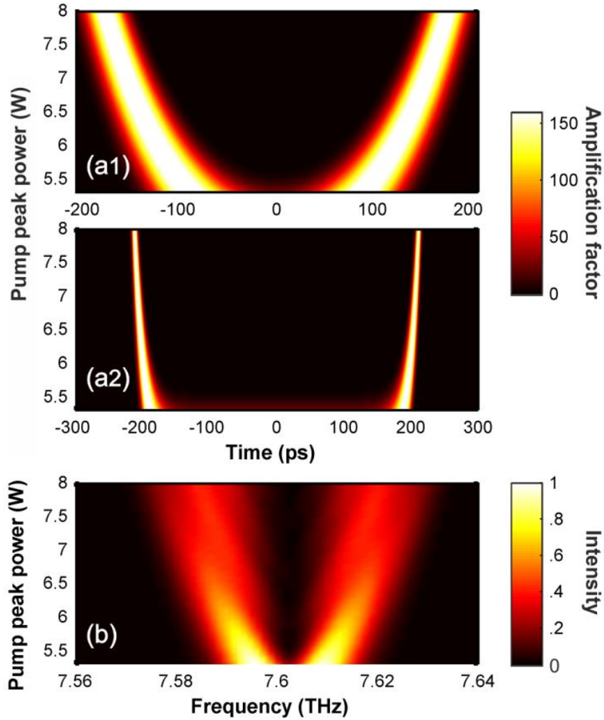
Figure 11 : (a) Evolution of the seed temporal intensity profile vs. the pump peak power for a (a1) Gaussian and a (a2) super-Gaussian pump profile. (b) Evolution of the seed spectral intensity profile vs. the pump peak power for a Gaussian pump profile.
