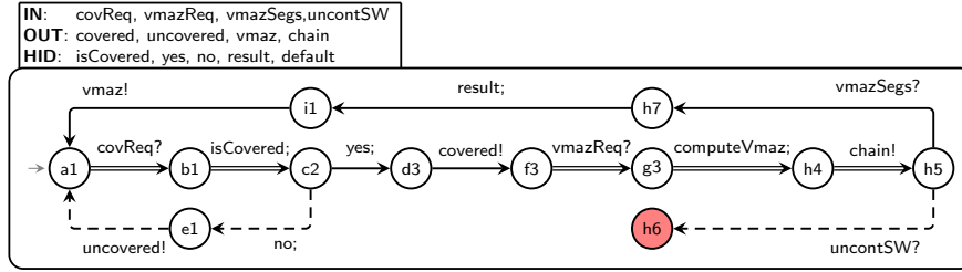
Figure 4: Interface automaton (B_d | B_m).\mathcal{A} .
