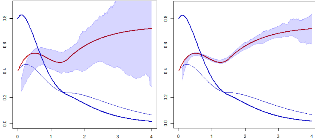
FIGURE 2. Reconstruction of B over \mathcal{D} = [0.1, 4] with 95%-level confidence bands constructed over M = 100 Monte-Carlo trees. In bold red line: x \rightsquigarrow B(x) ; in bold blue line: f_{H_B} ; in blue line: f_B . Left: T = 15 . Right: T = 23 .
