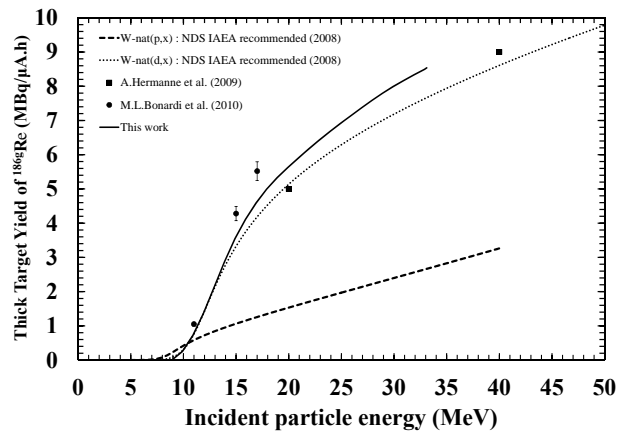
Figure 9: Comparison of the thick target yields of ^{186g}\text{Re} in MBq/ \mu\text{A}\cdot\text{h}
