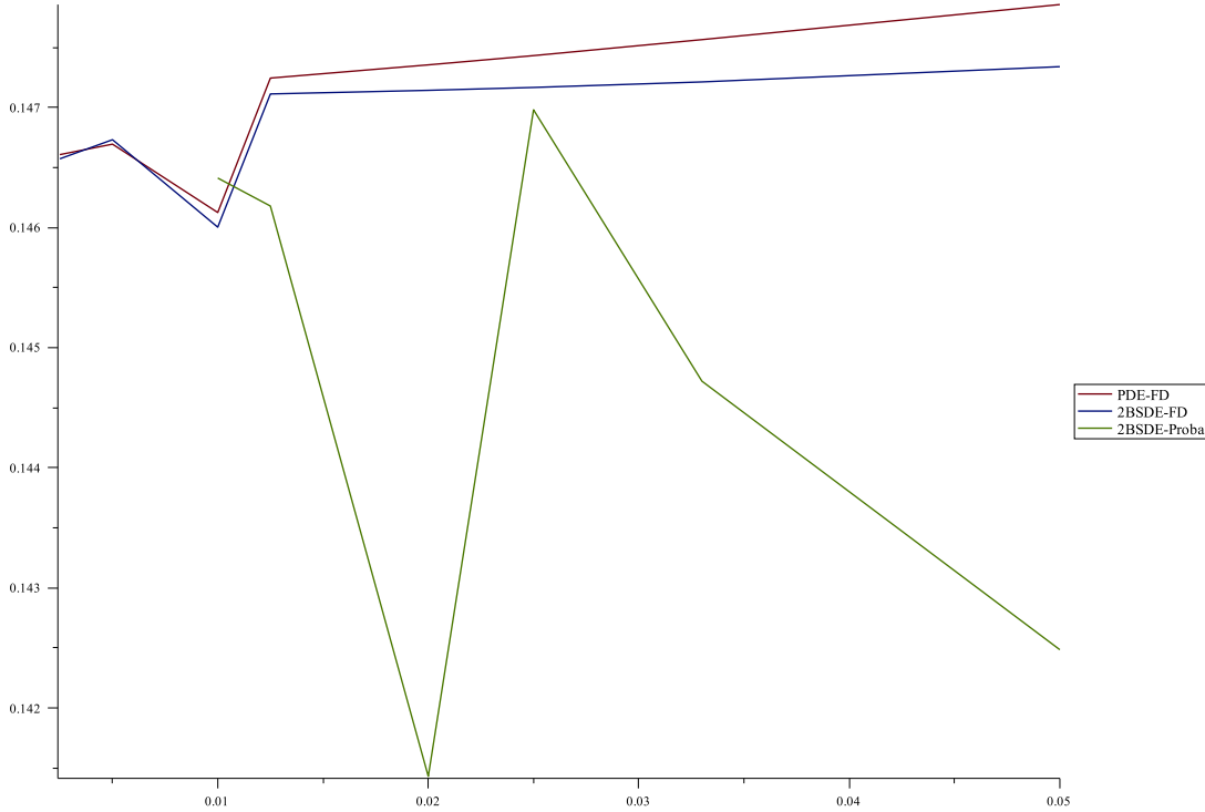
Figure 1: The comparison of numerical solutions for 2BSDE with generator (3.8). The faire value should be very closed to 0.146, and the probabilistic scheme seems more volatile comparing to the other schemes.
