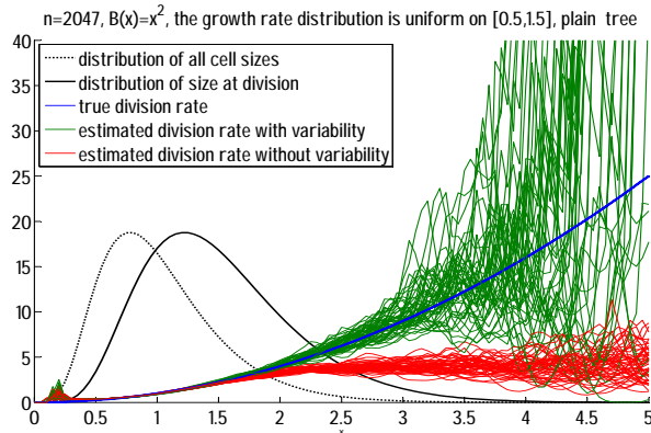
FIGURE 1. Simulated data: for N = 2047 we see the quality of \hat{B}_n over 50 Monte-Carlo simulations. The true B is in solid blue, and the Monte-Carlo reconstructions are in green. The reconstruction is fairly good in the region where the density \nu_B (in solid black) is not too small, and it consistently deteriorates beyond x \approx 3 , where almost no data of size x \geq 3 were observed. Note however the dramatic effect of ignoring variability (the Monte-Carlo estimators in red) beyond x \approx 2.5 .
