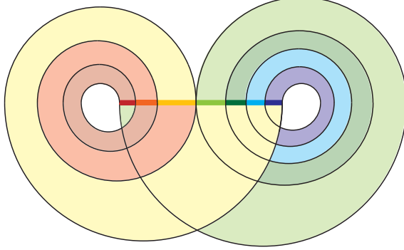
FIGURE 6. Division of the axis of \mathcal{T}_{p,q,r} into segments corresponding to orbits starting with a^3b, a^2b, ab, ba, b^2a, b^3a, and b^4a here.
