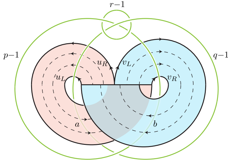
FIGURE 3. The template \mathcal{T}_{p,q,r} in T^1\mathbb{H}^2/G_{p,q,r} . The 3-manifold T^1\mathbb{H}^2/G_{p,q,r} is obtained from \mathbb{S}^3 by surgeries on a three-components Hopf link (green) with the given indices. The template \mathcal{T}_{p,q,r} is characterized by its embedding in T^1\mathbb{H}^2/G_{p,q,r} and by the kneading sequences that describe the orbits of the extremities of the ribbons. In case r is infinite, T^1\mathbb{H}^2/G_{p,q,r} is the open manifold obtained by removing the topmost component of the link. In the case p = 2 , the exit side of the left ribbon is strictly included into the entrance side of the right ribbon.
