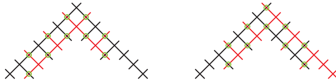
FIGURE 7. Crossing number between two orbits of codes a^ib^j (red) and a^{i'}b^{j'} (black), with i < i', j < j' on the left and i \leq i', j \geq j' on the right. The double points are encircled, they are 2(i + j) on the left and 2(i + j' - 1) on the right.
