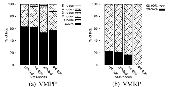
Figure 12. Improvement as compared to FFD
