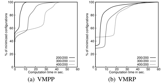
Figure 11. Impact of the ratio of VMs per node on the solving process
