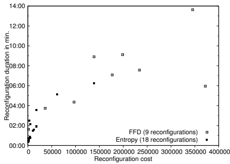
Figure 14. Reconfiguration costs computed by FFD and Entropy
