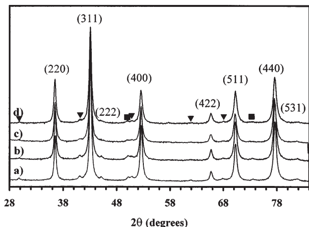
FIG. 2. XRD patterns of the Co-containing spinels (OCox): (a) x = 0.1 ; (b) x = 0.2 ; (c) x = 0.3 ; (d) x = 0.4 . Indexed peaks are those of the spinel phase. ( \nabla ) \alpha - \text{Al}_2\text{O}_3 contamination from the attrition balls; ( \blacksquare ) MgO.
