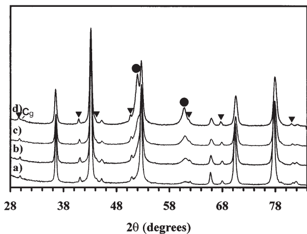
FIG. 6. XRD patterns of the Ni-containing nanocomposite powders after treatment with H_2-CH_4 at 1070^\circ C (Ni x ): (a) x = 0.1 ; (b) x = 0.2 ; (c) x = 0.3 ; (d) x = 0.4 . (●) Ni; (▼) \alpha-Al_2O_3 contamination from the attrition balls. Cg corresponds to d_{002} in multiwall nanotubes and/or in graphite; other peaks: spinel matrix.
