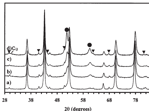
FIG. 5. XRD patterns of the Co-containing nanocomposite powders after treatment with \text{H}_2 - \text{CH}_4 at 1070 °C ( \text{Co}_x ): (a) x = 0.1 ; (b) x = 0.2 ; (c) x = 0.3 ; (d) x = 0.4 . ( \bullet ) \epsilon -Co; ( \nabla ) \alpha - \text{Al}_2\text{O}_3 contamination from the attrition balls. Cg corresponds to d_{002} in multiwall nanotubes and/or in graphite; other peaks: spinel matrix.
