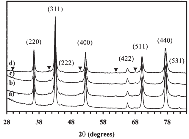
FIG. 1. XRD patterns of the Fe-containing spinels (OFe x ): (a) x = 0.1 ; (b) x = 0.2 ; (c) x = 0.3 ; (d) x = 0.4 . Indexed peaks are those of the spinel phase. (▼) \alpha -Al 2 O 3 contamination from the attrition balls.
