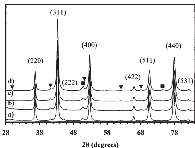
FIG. 3. XRD patterns of the Ni-containing spinels (ONix): (a) x = 0.1 ; (b) x = 0.2 ; (c) x = 0.3 ; (d) x = 0.4 . Indexed peaks are those of the spinel phase. ( \nabla ) \alpha - \text{Al}_2\text{O}_3 contamination from the attrition balls; ( \blacksquare ) NiO.
