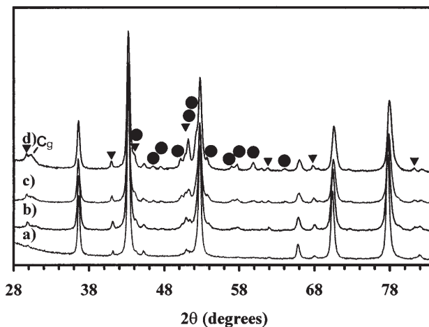
FIG. 4. XRD patterns of the Fe-containing nanocomposite powders after treatment with \text{H}_2 - \text{CH}_4 at 1070 °C ( \text{Fe}_x ): (a) x = 0.1 ; (b) x = 0.2 ; (c) x = 0.3 ; (d) x = 0.4 . ( \bullet ) \text{Fe}_3\text{C} ; ( \nabla ) \alpha - \text{Al}_2\text{O}_3 contamination from the attrition balls. Cg corresponds to d_{002} in multiwall nanotubes and/or in graphite; other peaks: spinel matrix. The \alpha -Fe (110) peak is masked by the (400) spinel peak at 2\theta equal to about 52^\circ .
