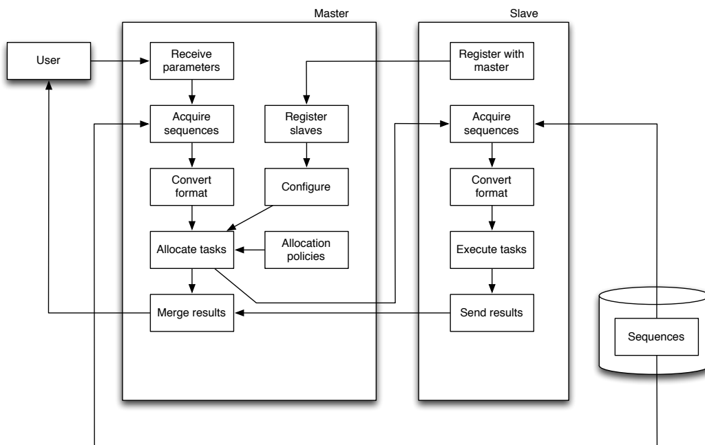
Figure 6. SWDUAL master-slave model
