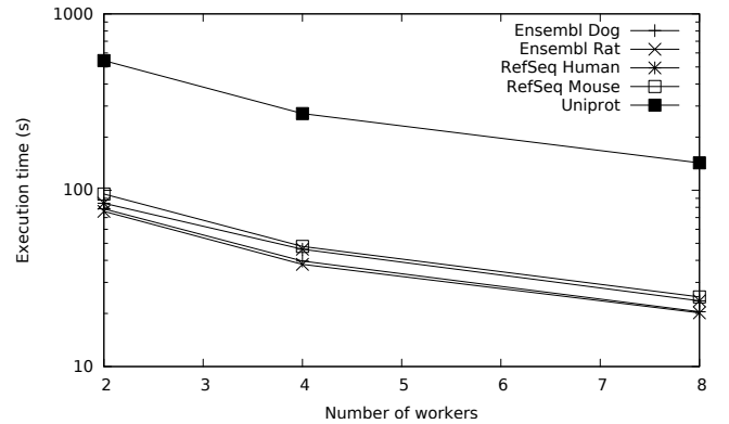
Figure 8. Execution times for the compared databases
