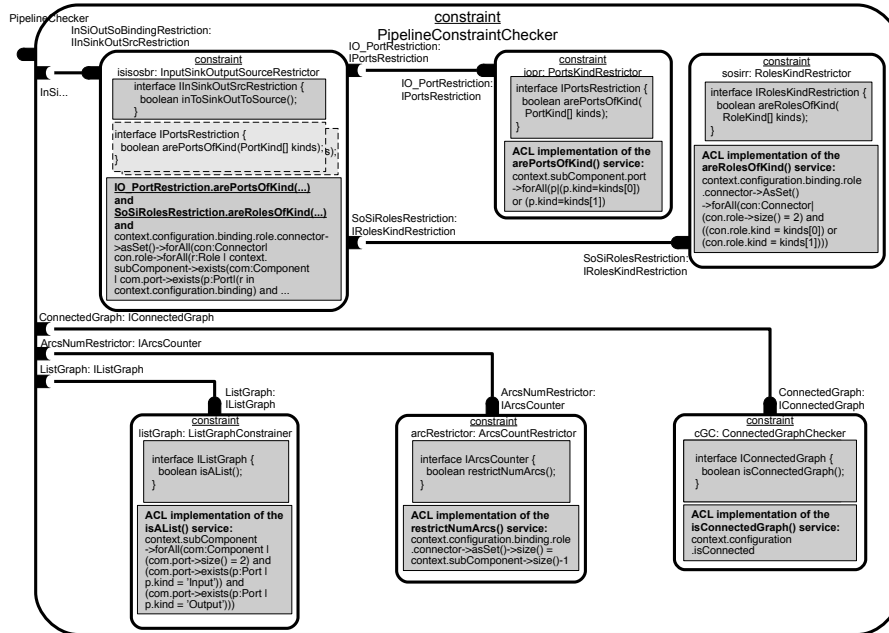
Figure 4: Architectural constraint composition (Figure taken from <26>)
