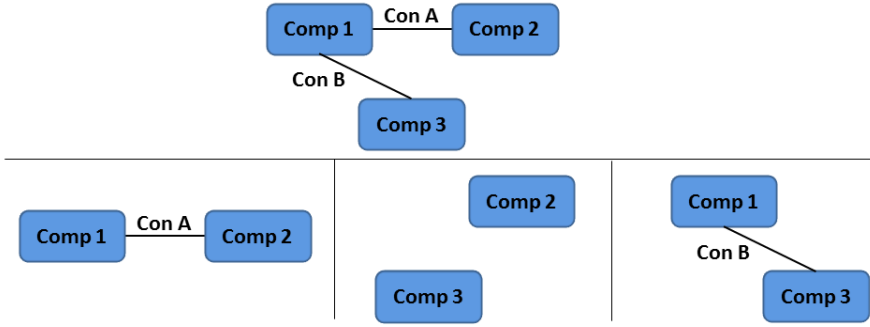
Fig. 18 Example of meaningful deletions
