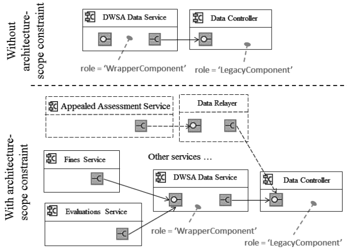
Fig. 11 StAD views for the Legacy Wrapper pattern produced from FRC architecture (Elements in dashed line are those added after the evolution of the FRC architecture)
