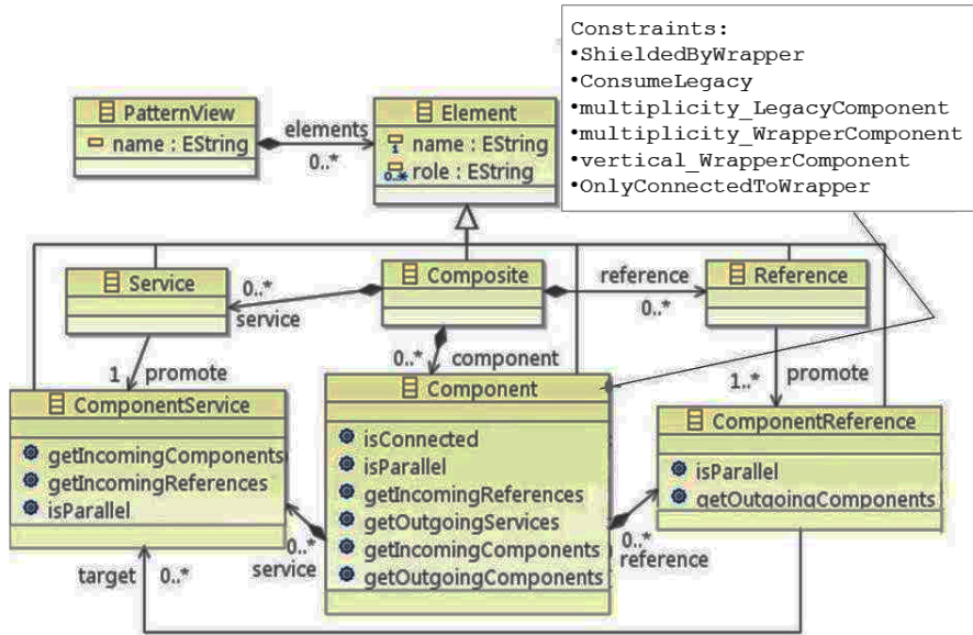
Fig. 12 StAD view meta-model for the Legacy Wrapper pattern.
