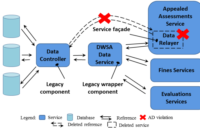
Fig. 3 Architectural decision violation by deletion
