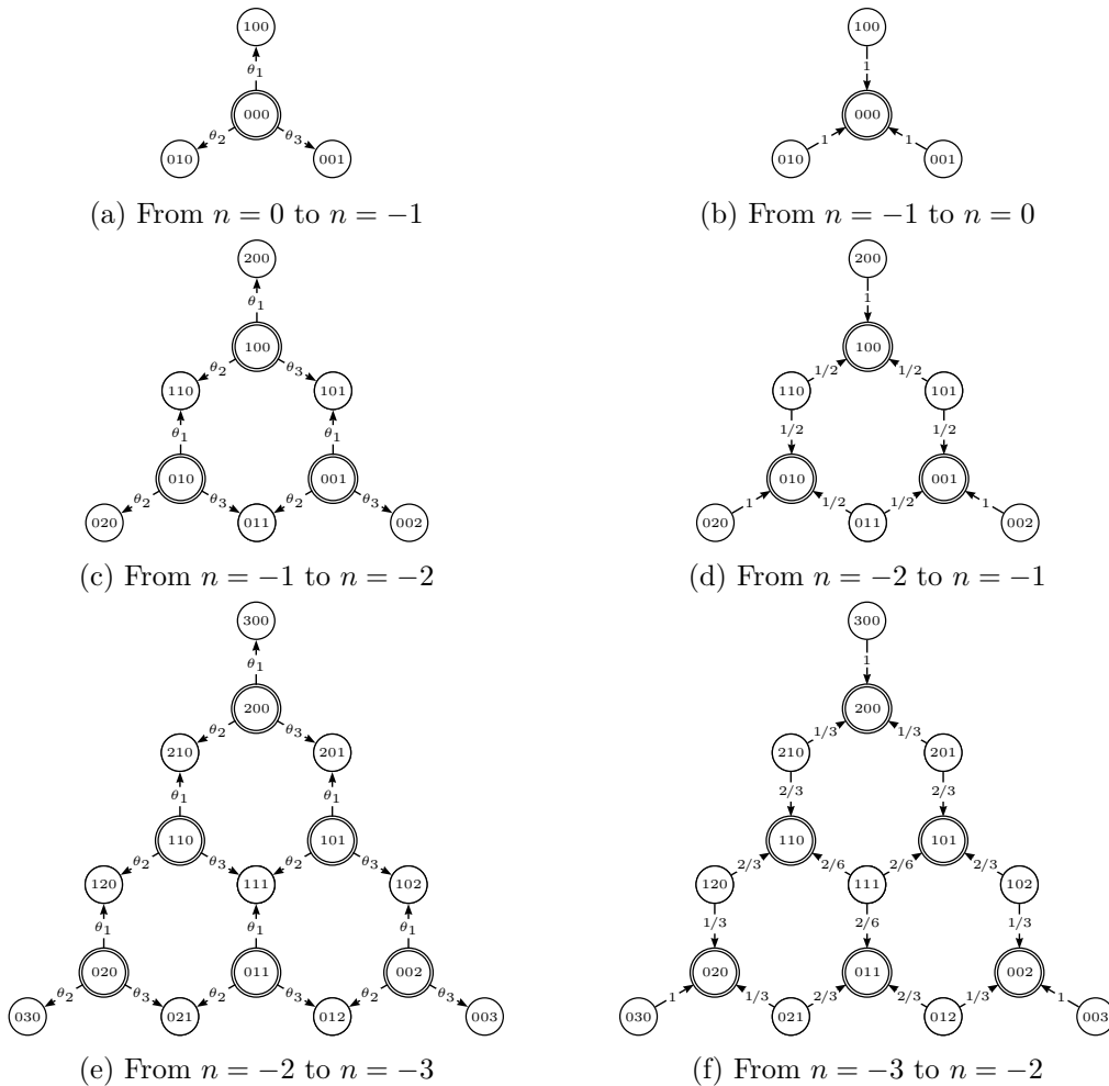
Figure 8: Random walk on the Pascal pyramid ( d = 3 )
