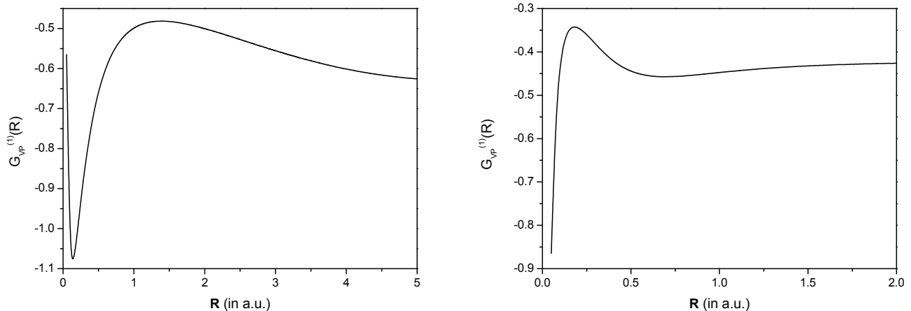
FIG. 2: "Effective potentials" G_{\text{VP}}^{(1)}(R) for the hydrogen molecular ions, Z_1 = Z_2 = 1 (left), and antiprotonic helium, Z_1 = 2 , Z_2 = -1 (right).
