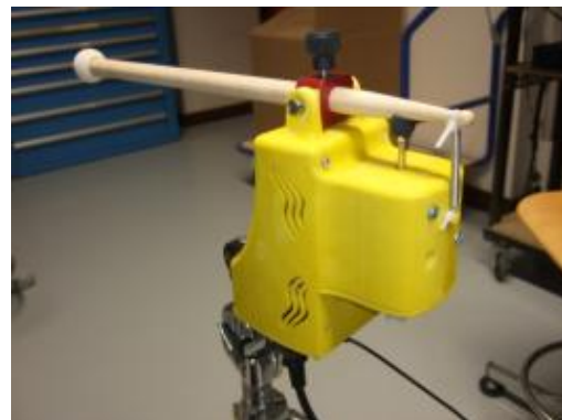
Fig. 5. z-printed housing
