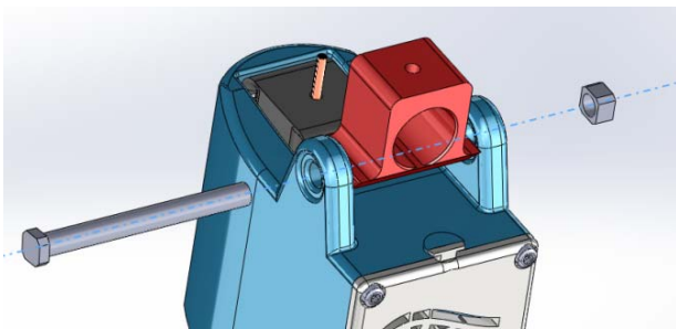
Fig. 3. Pin's assembly.
