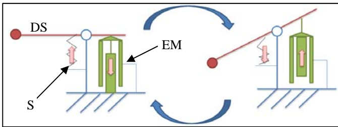
Fig. 2. Illustration of the lever (EM: electromagnet; S: spring; DS: drumstick).
