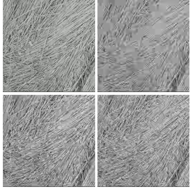
Fig. 3. Effect of replacing both SATD and SSD with SSIM and STSIM, QP value 51. Top left: Original Image, top right: encoded using default distortion measure, down left: SSIM instead of SATD and SSD, down right: STSIM instead of SATD and SSD
