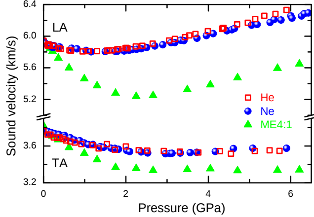
Figure 5: Sound velocities of v -SiO 2 as a function of P immersed in Ne (blue dots), He (red squares), 7 and ME4:1 (green triangles). 7 LA and TA denote the longitudinal and transverse acoustic velocities, respectively.
