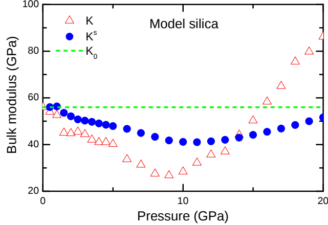
Figure 1: Pressure dependence of the bulk modulus of model silica (red triangles). 28 Blue dots are the secant bulk modulus used in the poromechanical model and the green dashed line shows the P = 0 value K_0 .
