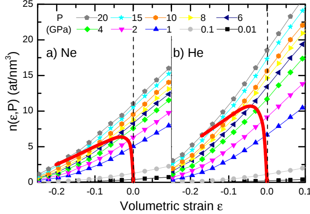
Figure 6: Room temperature adsorption isotherms in v -SiO 2 from GCMC simulations as a function of the bulk fluid pressure P : Ne (a), He (b). The symbols represent the calculated values whereas the thin lines are guides for the eye. The vertical dashed lines mark the unstrained volume. The bold red lines show the amount of gas-atoms adsorbed in silica predicted by the poroelastic constitutive equations in unjacketed conditions n^u(\epsilon^u, P) .
