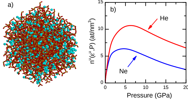
Figure 7: (a) Typical atomic configuration for He adsorbed at room temperature in silica glass at a bulk fluid pressure P = 6 GPa and a fixed volumetric strain \epsilon = -0.03 . To emphasize the large amount of adsorbed fluid atoms, about 11 \text{ at/nm}^3 , only He atoms are shown (blue spheres). The silica network is shown by sticks that are orange on the Si side and red on the O side. The simulation cube is projected along its [x, y, z] diagonal. (b) Pressure dependence of the amount of Ne and He atoms adsorbed by v\text{-SiO}_2 predicted by the poroelastic model in unjacketed conditions.
