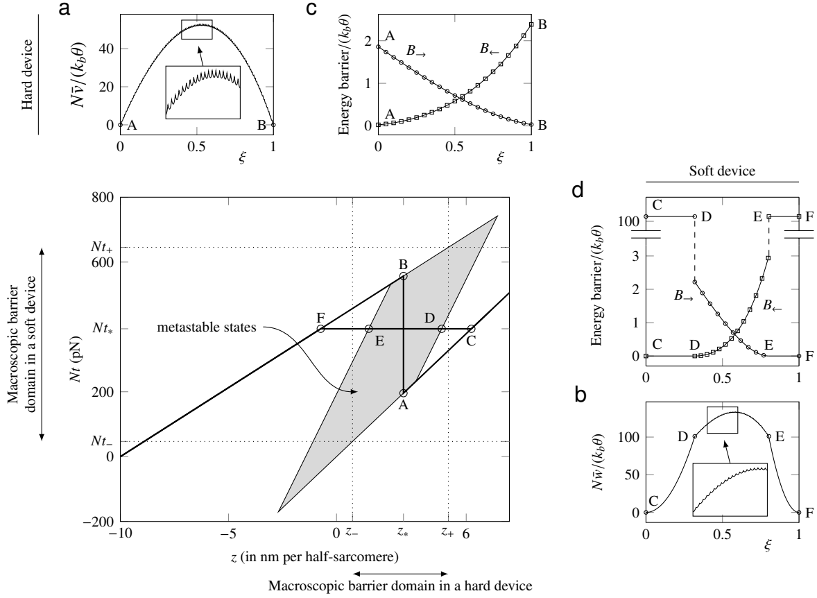
Figure 14: Result of the soft spin model with parameters adjusted to fit experimental data, see Caruel et al. (2013) . Main frame, tension-elongation relation for a single half-sarcomere. The gray area shows the existence domain of the metastable states. Solid lines, global minimum tension-elongation relation in hard and soft devices. (a) and (b), Energy landscape corresponding to single transition between the homogeneous states in a hard device ( A \rightarrow B ), see (a) and in a soft device ( C \rightarrow F ), see (b). (c) and (d) size of the energy barriers corresponding to the individual folding ( B_{\rightarrow} ) and ( B_{\leftarrow} ) transitions obtained with both finite N (open symbols) and in the thermodynamic limit (solid lines). To improve readability of the finite N plots, we only show one out of five micro-transition points.
