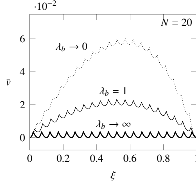
Figure 12: Energy landscape at the global minimum transition for the snap-spring model in a hard device at different values of the coupling parameter \lambda_b with N = 20 . [bold line, \lambda_b \rightarrow \infty ; solid line, \lambda_b = 1 ; dotted line, soft device limit as the hard device case where \lambda_b \rightarrow 0 , z_* \rightarrow \infty . Energy minima are arbitrarily set to 0 for comparison. Other parameters are as in Fig. 9.
