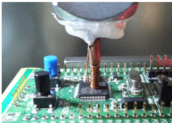
Fig. 1. EM bench: the chip and the probe.
