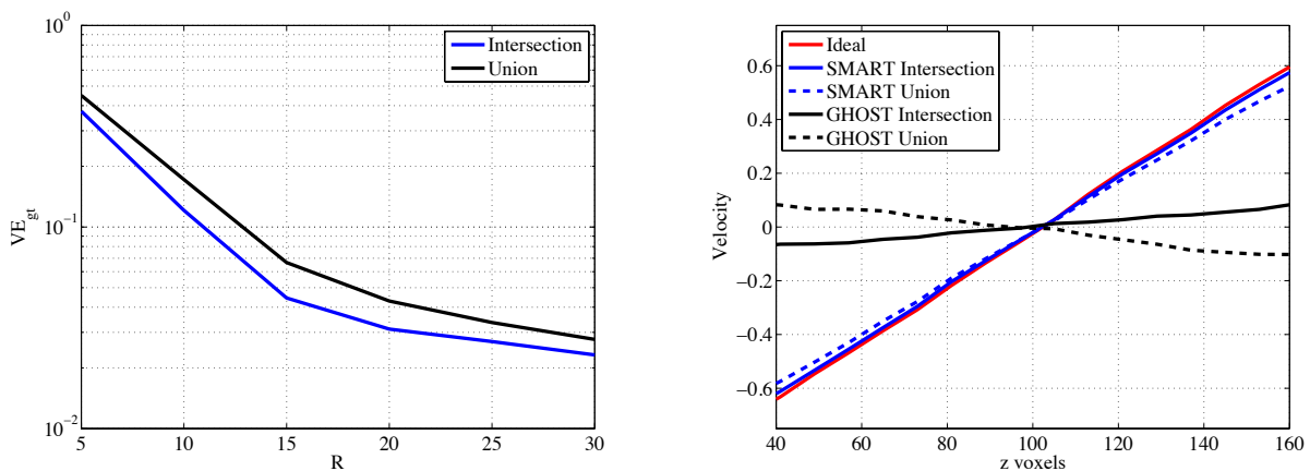
Fig. 5 Average velocity errors for \alpha=0.01 (left) as a function of the IVs radius R. Velocity profiles along Z, averaged in the X and Y directions (right) for ideal reconstruction, SMART reconstruction and ghost particles. Cases where particles lie only in the Intersection, or in the Union. On the right subfigure, the IV side is set to 41 voxels (radius of 20 voxels).
