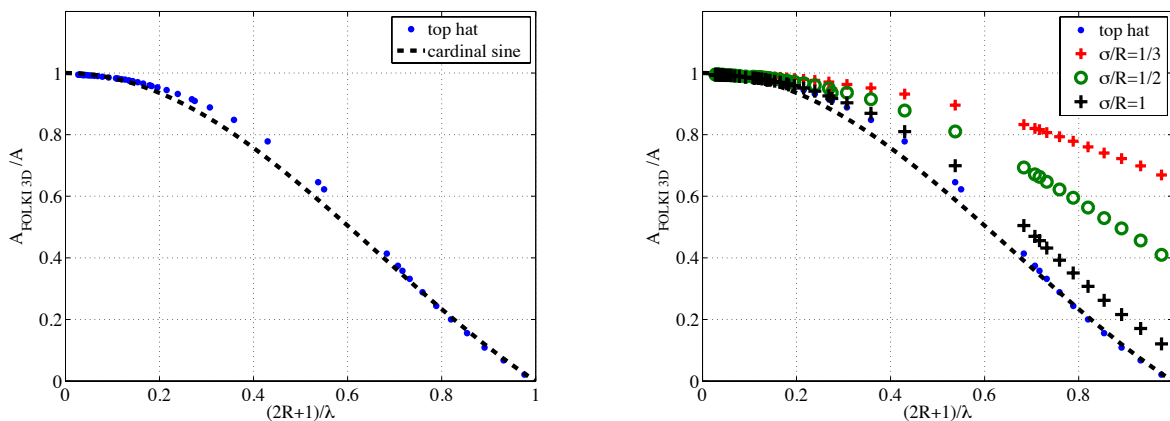
Fig. 1 Amplitude ratio A_{\text{FOLKI-3D}}/A as a function of the normalized volume interrogation size for (left) top hat IVs and (right) Gaussian IVs. The dashed line is the response of a [-R, R] sliding average (cardinal sine function)
