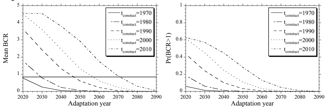
Figure 6. Effect of the adaptation year on the mean BCR and Pr(BCR>1) for slabs (D=300mm) built at several years in Saint-Nazaire, RCP 4.5 scenario and \Delta c_{adapt}=5 mm.
