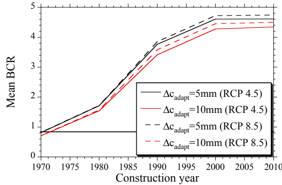
Figure 5. Mean BCR for slabs (D=300mm) built in several years in Saint-Nazaire and t_{adapt}=2020 .
