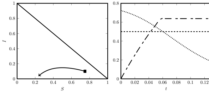
Fig. 3 The parameters used are (S_{0-}, I_{0-}) = (0.75, 0.1) , \beta = 73 , \gamma = 36.5 , r_I = 1 , r_V = 0.5 , u_{max} = 10 and constraint in Equation (19) f(t) = \frac{u_{max}}{S(t)} . Left: The trajectory (S(t), I(t)) of the system (1) with U = 0 . Right: The decreasing dotted curve is t \mapsto \frac{\varphi_I(\infty) - \varphi_I(t)}{1 - \varphi_I(t)} , the constant densely dashed line is the level r_V/r_I and the increasing dashed-dotted curve is the probability of vaccination over time.
