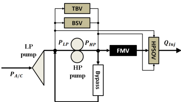
Figure 5: Complete system with ancillary valves where FMV means Fuel Metering Valve
