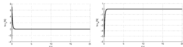
Fig. 7. Feedback tracking controller in the vertical plane
