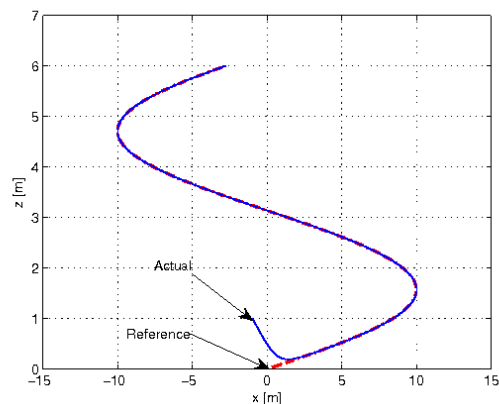
Fig. 5. Actual and reference trajectory in vertical plane
