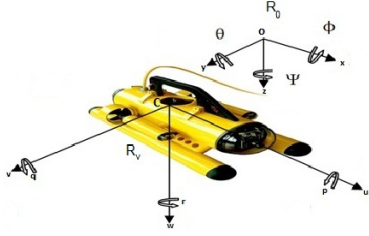
Fig. 1. Body-fixed frame and earth-fixed reference frame for the ROV
