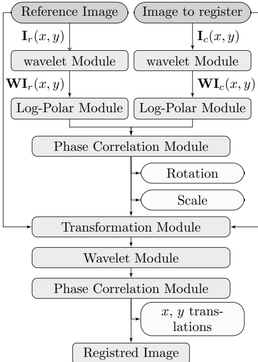
Figure 2: Overview of the registration algorithm.
