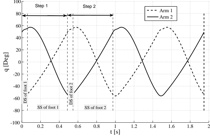
Figure 10: Evolution of arms versus time at walking speed V = 1 \text{ m/s}
