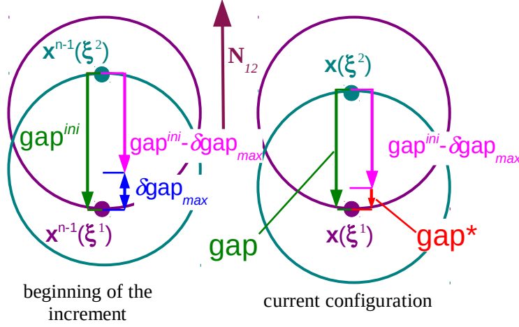
Figure 3: Definition of the modified gap used for the process of gradual reduction of gaps
