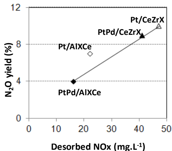
Figure 7: Relationship between, the N 2 O yield and the NO x desorption recorded during the rich pulses. NSR tests performed over FTM honeycomb supported catalysts at 300°C using the “full gas” mixture.
