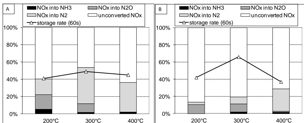
Figure 1: Percentage of stored NO x in 60s (Δ) and NO x storage/reduction efficiency in cycled condition at 200, 300 and 400°C with mixtures depicted in Table 1 (full gas) for Pt/CZ catalyst used as powder (A) and honeycomb (B).
