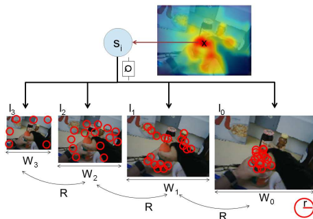
Figure 2: Representation of our Visual Fields with Variable Spatial Resolution and Non-uniform sampling
