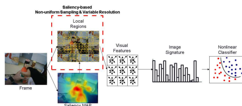
Figure 1: Processing pipeline for the saliency-based object recognition in first-person camera videos
