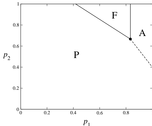
Figure 2. Phase diagram in the plane (p_1, p_2) according to mean-field approximation. The full circle, located at (p_1, p_2) = (5/6, 2/3) , corresponds to the voter model. The phases are: paramagnetic (P), ferromagnetic (F) and absorbing (A). The solid lines are continuous phase transitions and the dashed line is a discontinuous phase transition.
