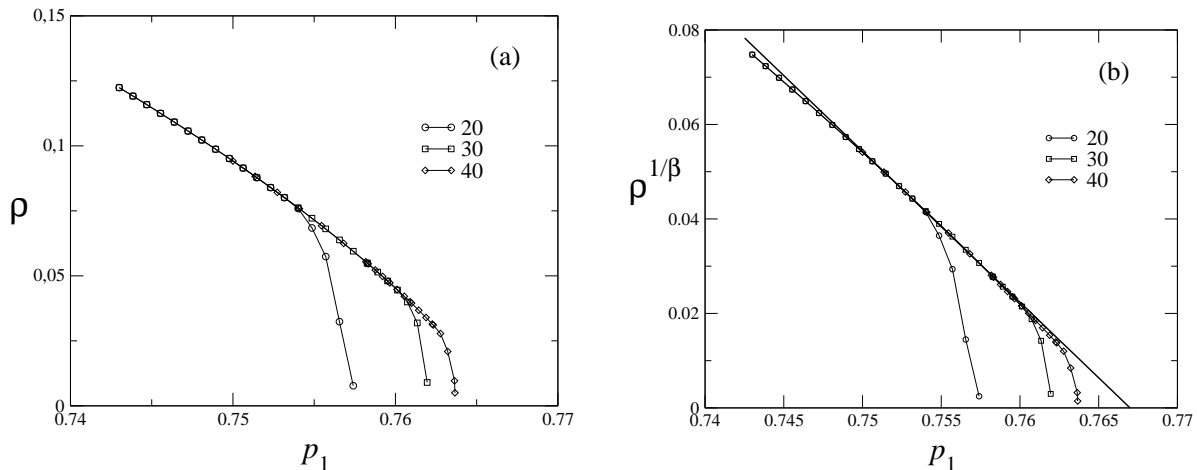
Figure 5. (a) Order parameter \rho of the F-A transition as a function of p_1 for p_2 = 1 . The critical point occurs at p_{DP} = 0.7670 as can be inferred from the plot (b) where \beta = 0.81
