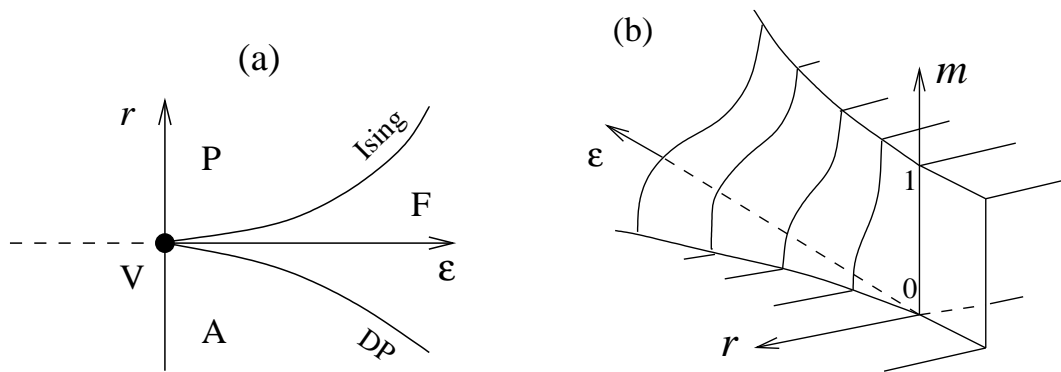
Figure 1. (a) Phase diagram in the field parameters \varepsilon and r . The full circle, located at the origin, corresponds to the voter model (V). The phases are: paramagnetic (P), ferromagnetic (F) and absorbing (A). The solid lines are continuous phase transitions belonging to the Ising and DP universality classes and the dashed line is a discontinuous phase transition. (b) Magnetization m as a function of \varepsilon and r .
