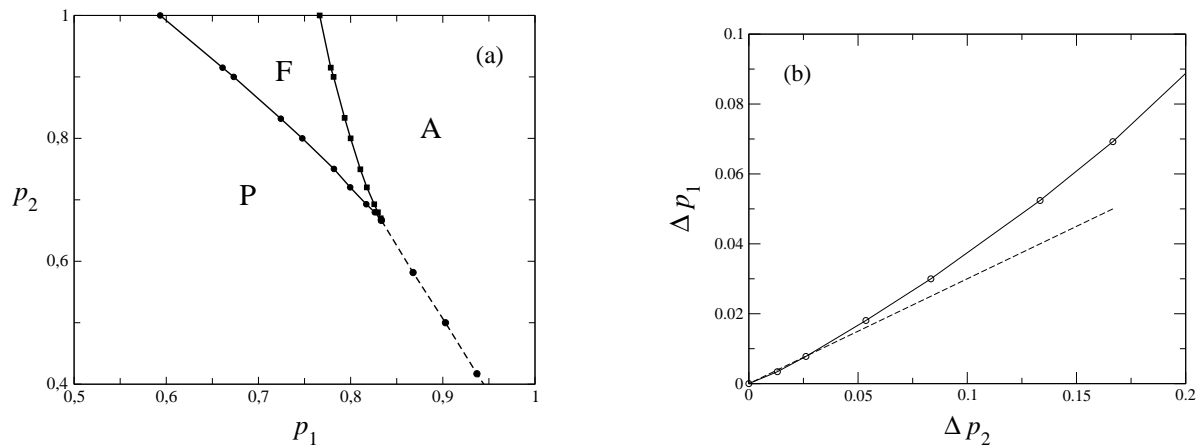
Figure 6. (a) Phase diagram in the plane (p_1, p_2) according to simulations on a cubic lattice. The phases are: paramagnetic (P), ferromagnetic (F) and absorbing (A). The solid lines are continuous phase transitions and the dashed line is a discontinuous phase transition. The three lines meet at the point (p_1, p_2) = (5/6, 2/3) , corresponding to the voter model. (b) Linear size \Delta p_1 = p_{FA} - p_{PF} of the ferromagnetic phase as a function of the distance from the voter point \Delta p_2 = p_2 - 2/3 . The dashed straight line shows that the data points have a finite slope at the origin.
