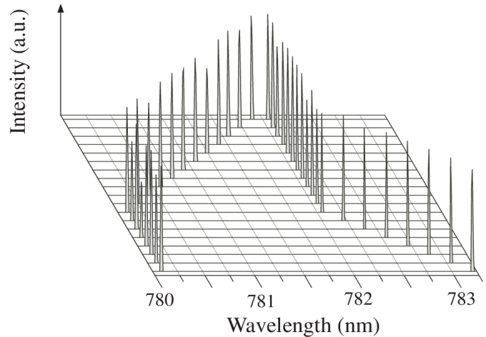
Fig. 4. Optical spectrum of the two-axis laser as one intracavity thin étalon is tilted while the second one is fixed. Note that each wavelength can be tuned independently. Res 0.01nm.
