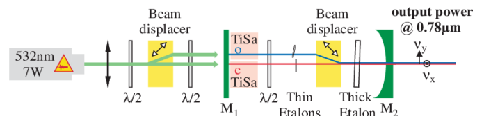
Fig. 1. Schematic diagram of the laser. \lambda/2 : half wave plate. M_1 : plane dichroic mirror, M_2 : 95% output coupler, o: ordinary axis, e: extraordinary axis.
